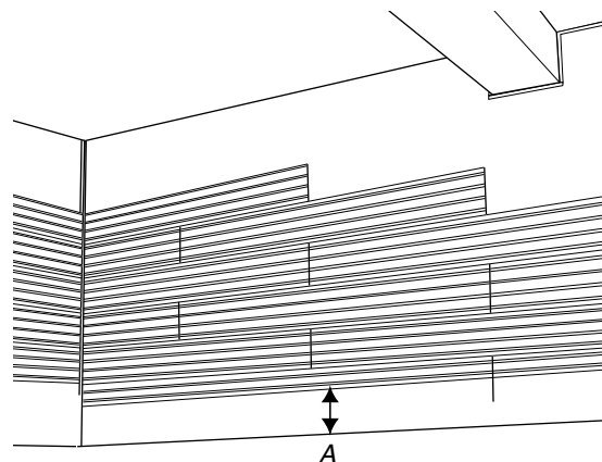
A. 12" (30.5 cm) between panel and floor
